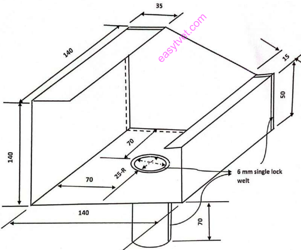
Gutter end cup Detail A.
