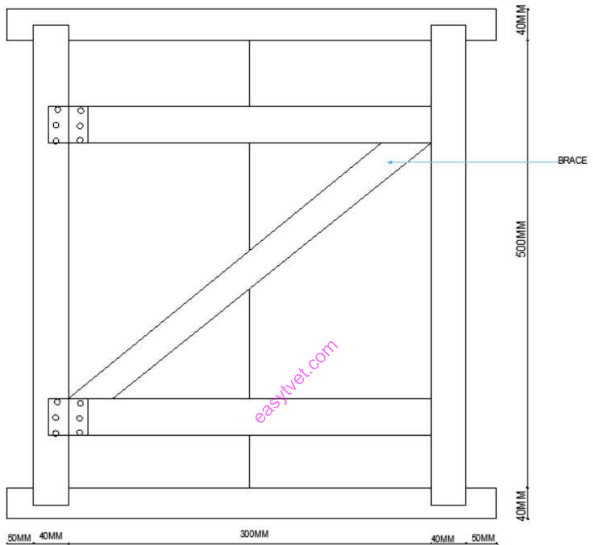
REAR ELEVATION
