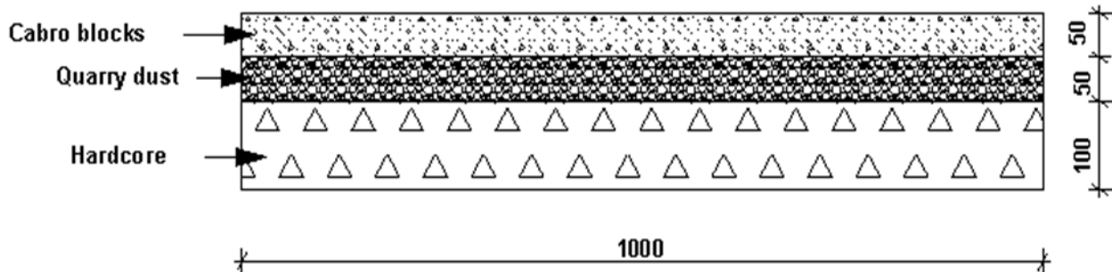
Sectional Drawing
