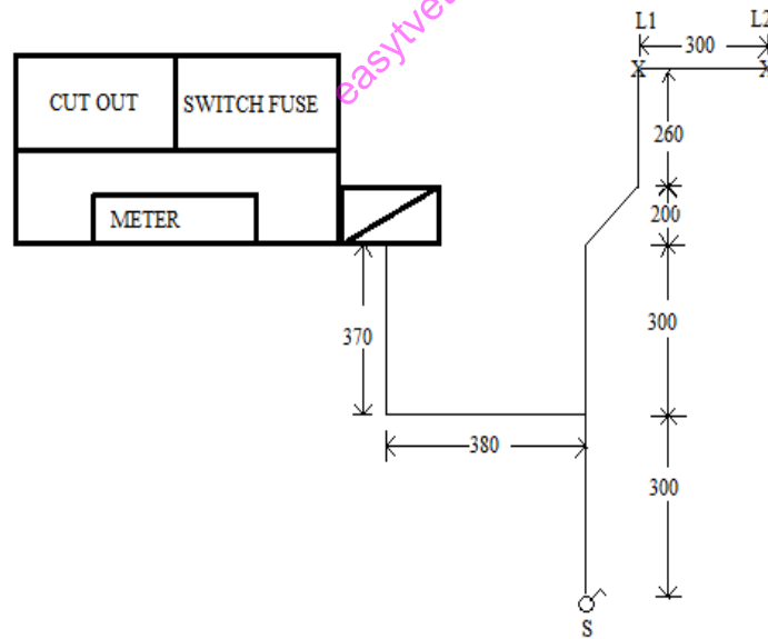
Figure 1: Layout diagram
