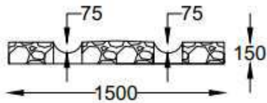
SECTION Z-Z
