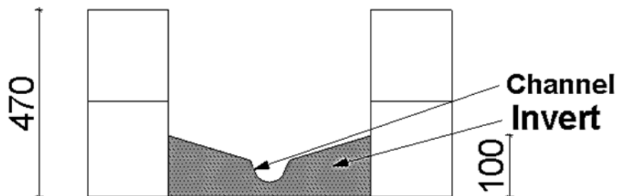
SECTION 01-01
