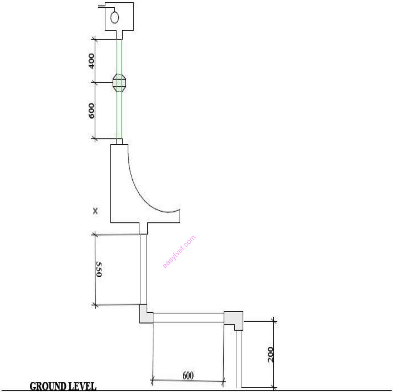
INSTALLATION OF BOWL URINAL
